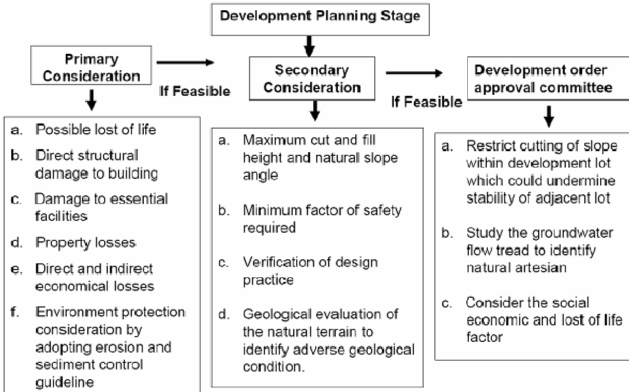
Figure 2. Some loss reduction factors to be considered during development planning stage.
